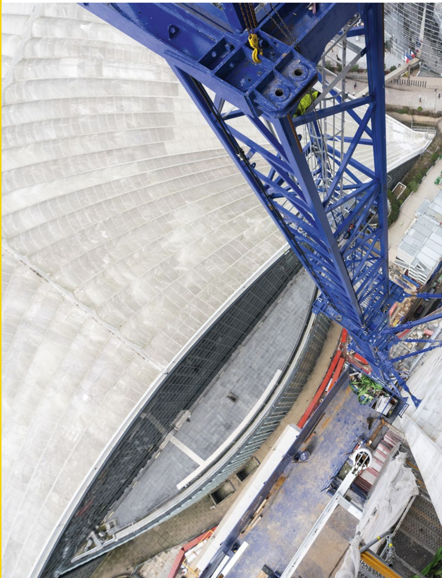
Repositioning the braces of a tower crane, France © 2019 - Petzl Distribution - Vuedici.org - Integral - Bateg - Tour Trinity - Cro&Co Architecture
